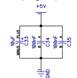
Decoupling Capacitors
