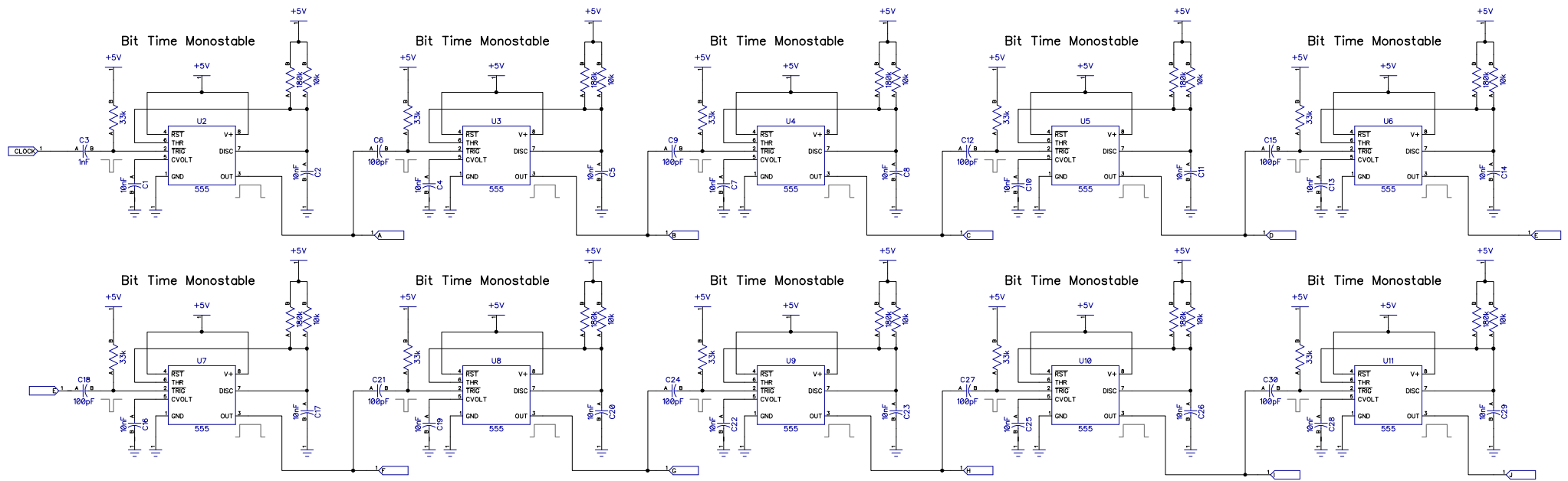
All 555 Asynchronous Serial Generator - Luc Small, February 2011
