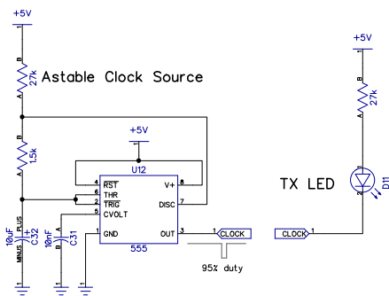
All 555 Asynchronous Serial Generator - Luc Small, February 2011
